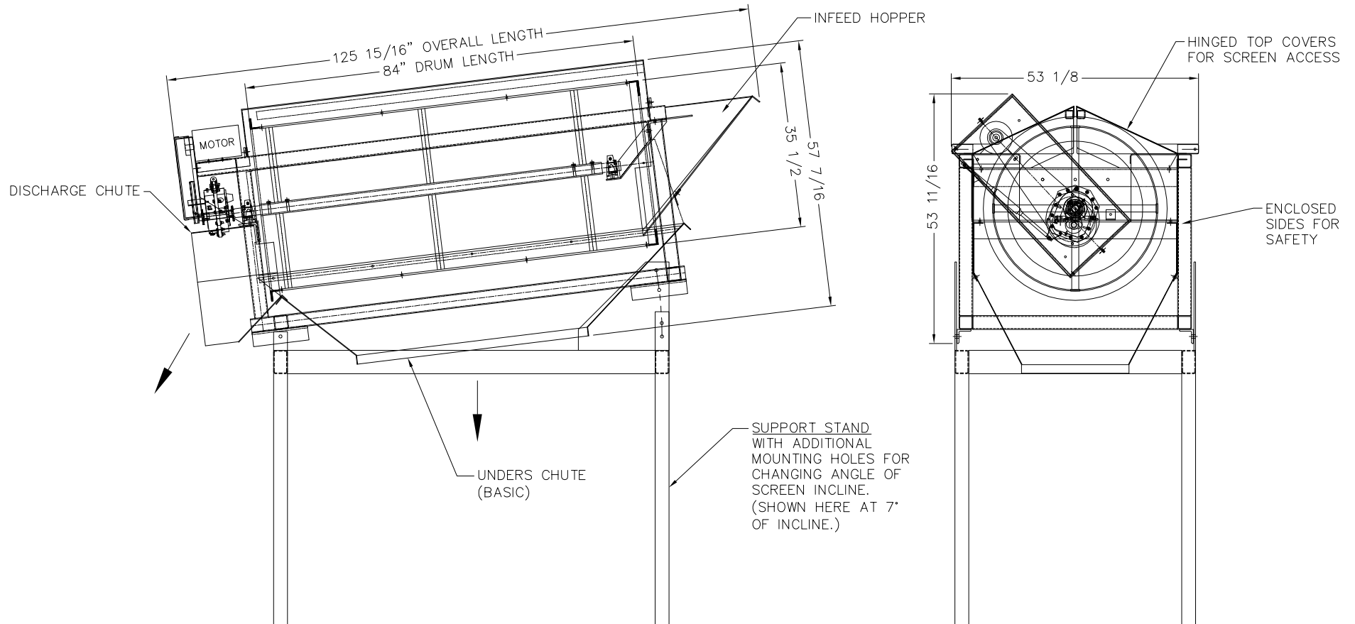
SIDE ELEVATION VIEW
